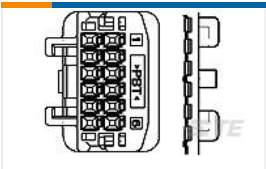
TE Part #1473410-1 025 G 16POS CAP ASSY W TO W
