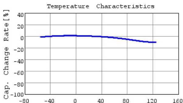
RCER71E154K0DBH03A C-Temp. capchange, DC0.0V
