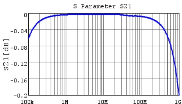
RCER71E154K0DBH03A S21 DC0V, 25degC
