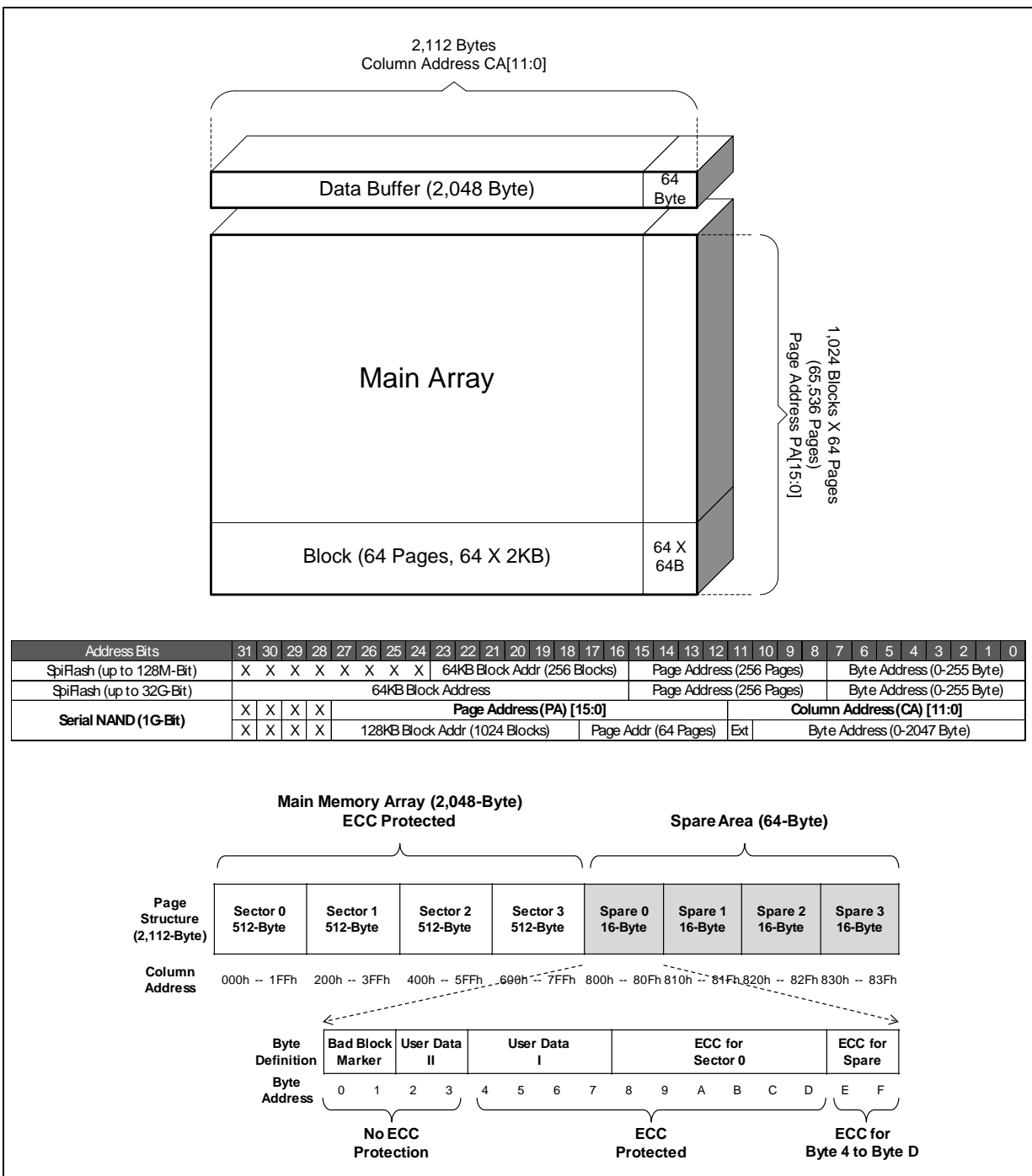
Figure 2b. Single Die W25N01GW Flash Memory Architecture and Addressing
