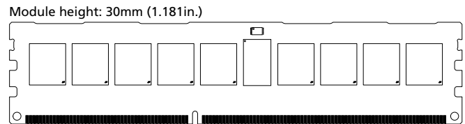
Figure 1: 240-Pin RDIMM (MO-269 R/C B1)
