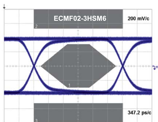
Figure 12. USB2.0 480 Mbps eye diagram with device
