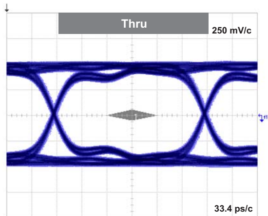
Figure 13. USB3.0 5 Gbps eye diagram without device
