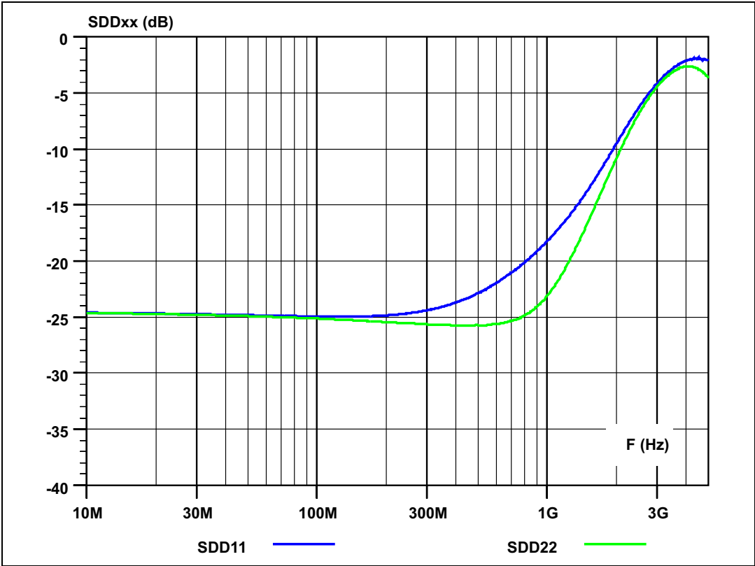
Figure 5. Return loss versus frequency ( Z_0 \text{ com} = 50 \Omega )
