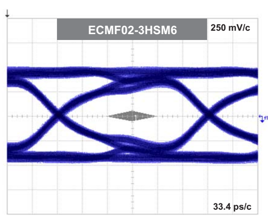
Figure 14. USB3.0 5 Gbps eye diagram with device
