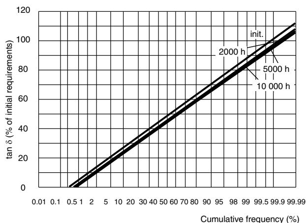
Fig. 11 - \tan \delta change of capacitance as a function of cumulative frequency after endurance test
