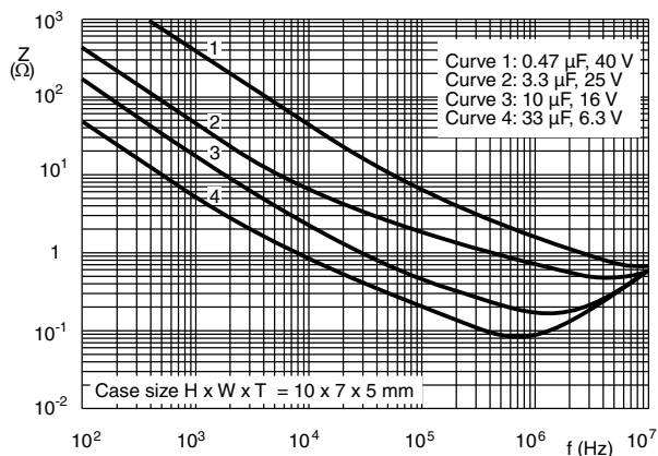
Fig. 21 - Typical impedance at 25 °C as a function of frequency
