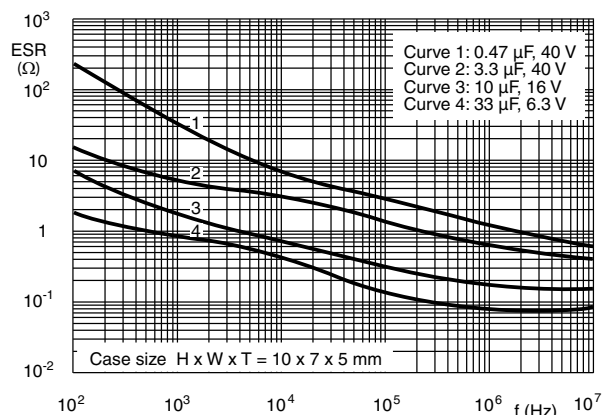
Fig. 15 - Typical ESR at 25 °C as a function of frequency
