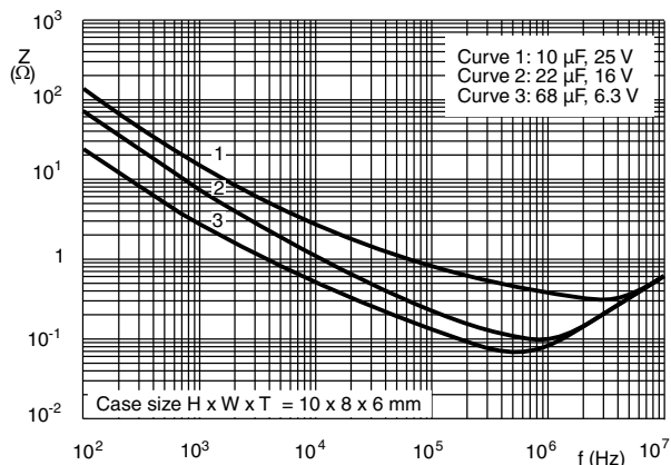
Fig. 23 - Typical impedance at 25 °C as a function of frequency
