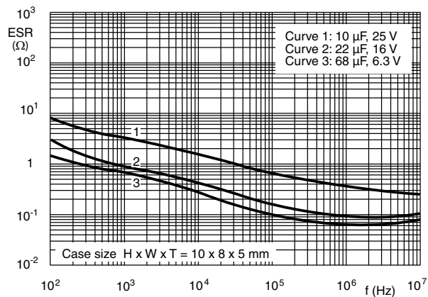
Fig. 17 - Typical ESR at 25 °C as a function of frequency
