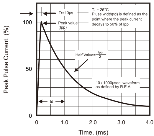
Fig.5 - Pulse Waveform
