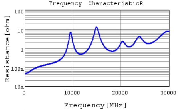
GJM0335C1H9R4CB01 R DC0V, 25degC
