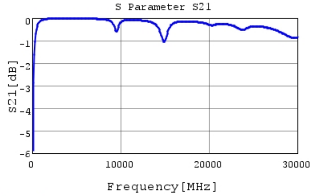
GJM0335C1H9R4CB01 S21 DCOV, 25degC
