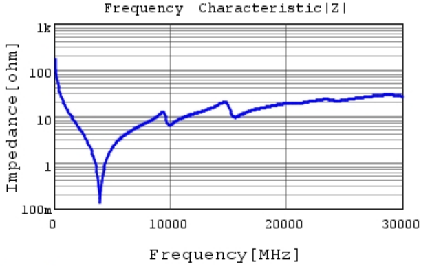
GJM0335C1H9R4CB01 |Z| DC0V, 25degC
