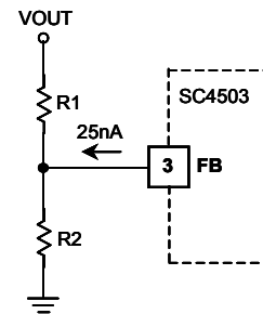
Figure 3. R_1 - R_2 Divider Sets the Output Voltage
