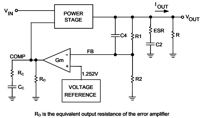
Figure 6. Simplified Equivalent Model of a Boost Converter
