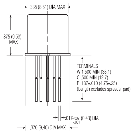
1MST Enclosure
