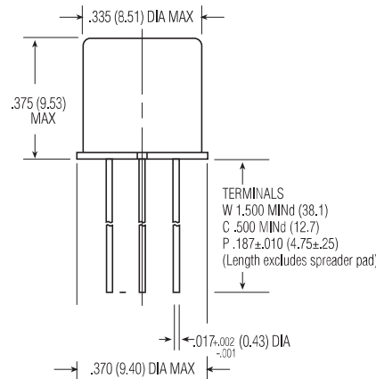
1MS/1MSD/1MSDD Enclosure
