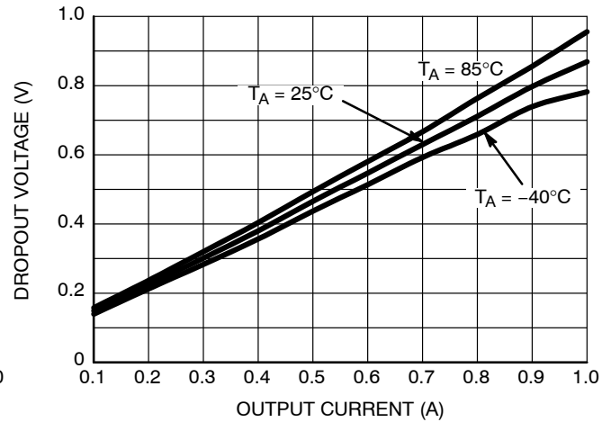
Figure 16. Dropout Voltage vs. Output Current NCP693xMN12TCG
