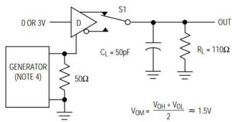
Drive enable and disable time
