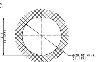
Panel Drilling
