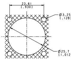
Panel Drilling
