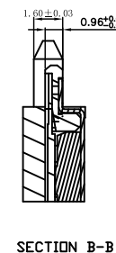
SECTION B-B
