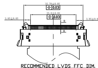
RECOMMENDED LVDS FFC DIM.
