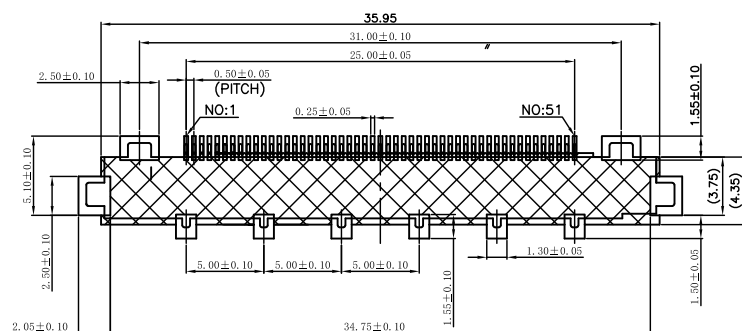
RECOMMEND P.C.B LAYOUT SCALE 1:2
