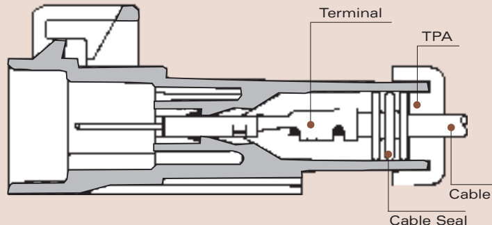
Male Connector
