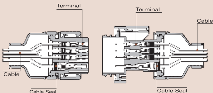
Female Connector Assembly
