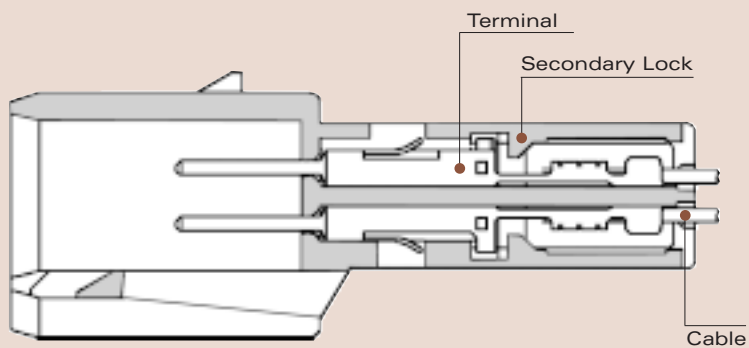
Male Connector
