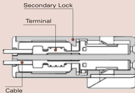
Female Connector
