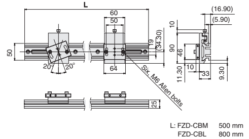
3D Camera Base FZD-CBM/CBL
