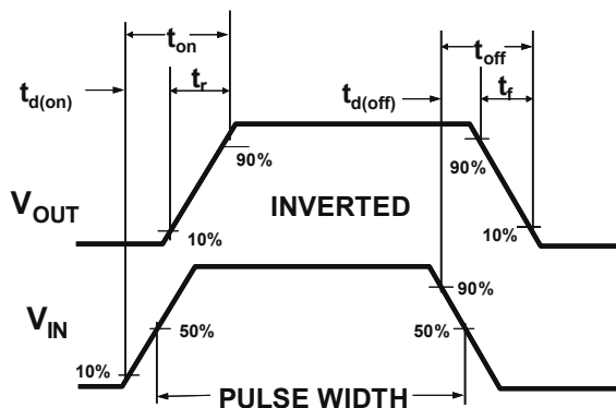
Figure 2: Switching Waveforms
