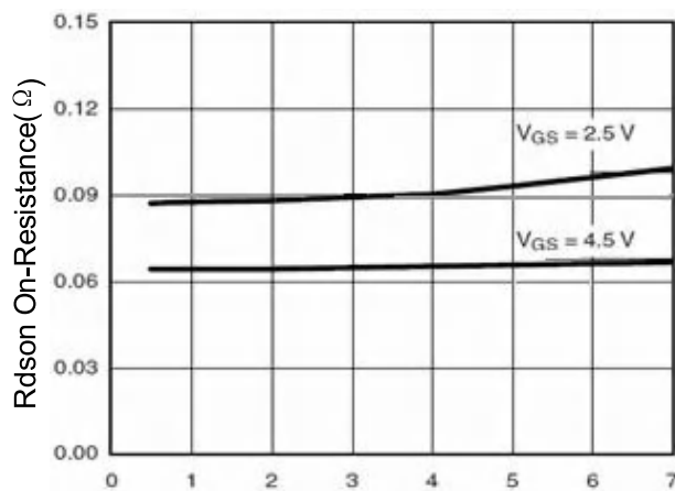
Figure 6 Drain-Source On-Resistance
