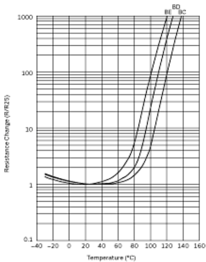
Resistance - Temperature Characteristics
