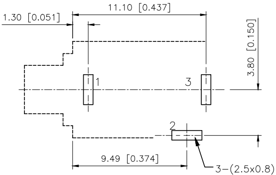
PCB Layout
