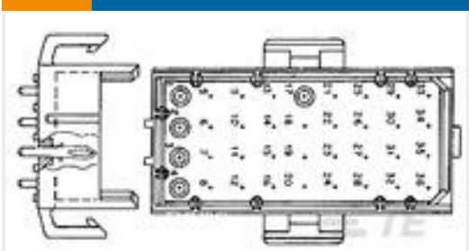
TE Part #640500-2 06P MR HDR ASSY V0
