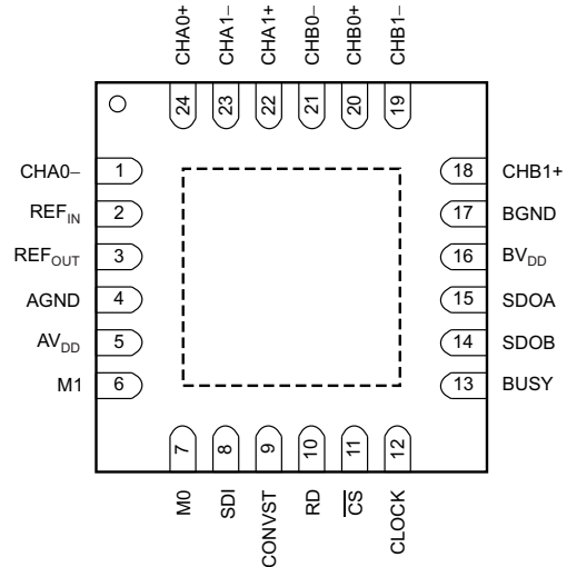
RGE PACKAGE 4-mm × 4-mm QFN-24 (TOP VIEW)
