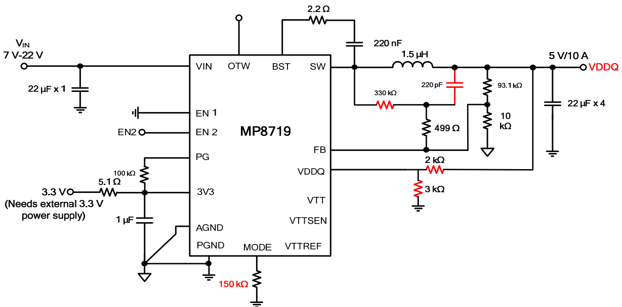
Figure 17: Special Application Circuit, V_{IN} = 7\text{V} - 22\text{V} , V_{OUT} = 5\text{V} , I_{OUT} = 10\text{A} , f_s = 700\text{kHz}
