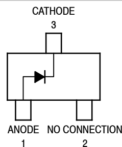
SC-70 (SOT-323) CASE 419 STYLE 2
