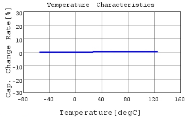
KRM55R5C2J223JDL1 C-Temp. capchange, DCOV, 1
