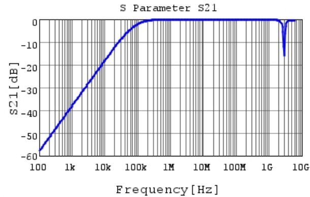
KRM55R5C2J223JDL1 S21 DCOV, 25degC
