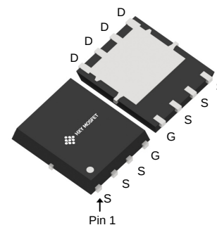
DFN5X6-8L (DFN-8(5.2x5.9))
