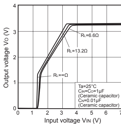
Fig.5 Output Voltage vs. Input Voltage (Typical Value) (PQ1M335M2SPQ)
