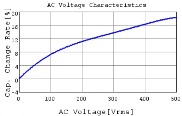
DE1B3RA101KJ4BQ01F C-AC Voltage capchange, 1
