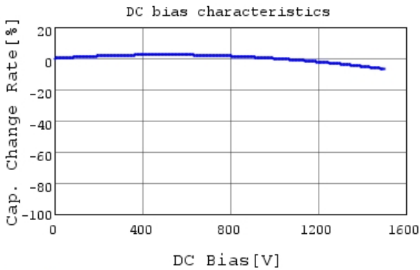
DE1B3RA101KJ4BQ01F C-DC bias capchange, 20.0
