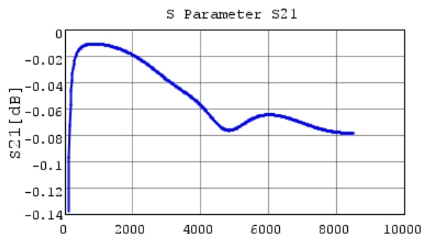
GRM0225C0J910GA02 S21 DCOV, 25degC
