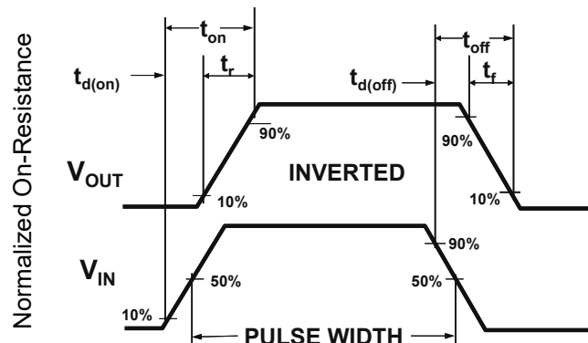
Figure 2: Switching Waveforms
