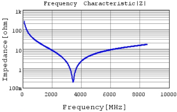
GCQ1555C1H6R2CB01 |Z| DC0V, 25degC
