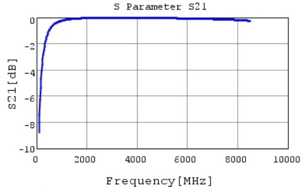
GCQ1555C1H6R2CB01 S21 DCOV, 25degC
