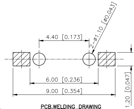
PCB.WELDING DRAWING
