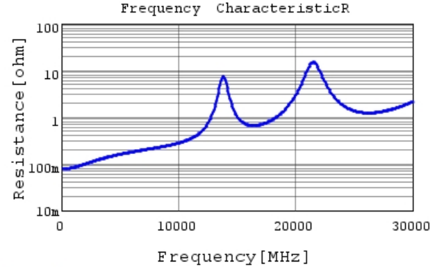
GJM0335C2A5R2CB01 R DCOV, 25degC
