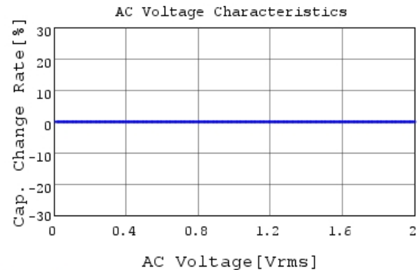
GJM0335C2A5R2CB01 C-AC Voltage capchange, Dc
