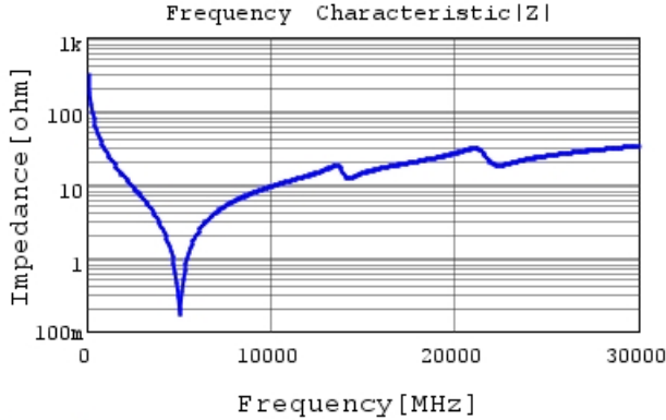
GJM0335C2A5R2CB01 |Z| DCOV, 25degC
