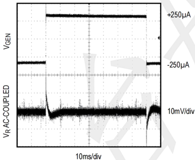
LOAD-TRANSIENT RESPONSE
