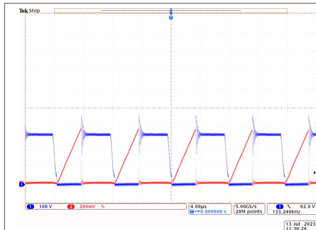
Figure 8-2. V_{IN} = 115 \text{ VAC} V_{OUT} = 20 \text{ V} I_{OUT} = 3.25 \text{ A}
