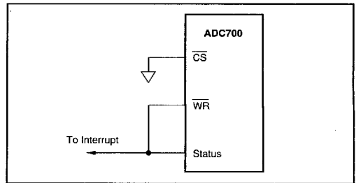
FIGURE 11. Continuous Conversion Circuit Connection.
