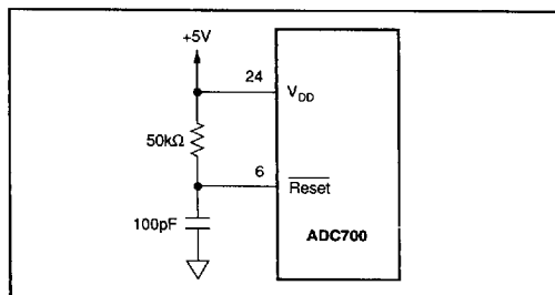
FIGURE 8. Power-Up Reset Circuit.
