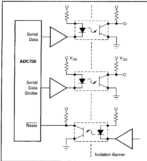
FIGURE 10. Serial Data Output Providing Convenient Isolation.
