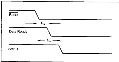
ADC700 Reset Function Timing Diagram.
