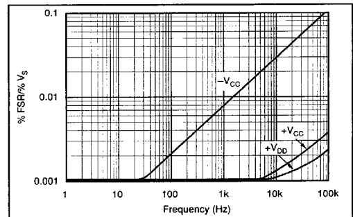
FIGURE 4. Power Supply Rejection Ripple vs Frequency.
