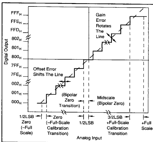
FIGURE 3. Transfer Characteristic Terminology.
