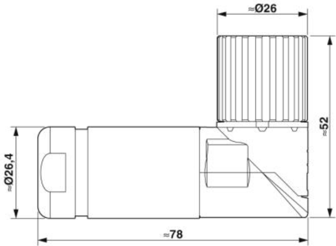
Dimensional drawing
