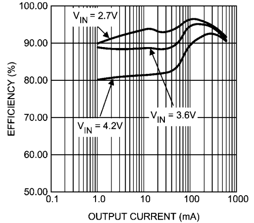
BUCK 2 Efficiency vs Output Current (PFM to PWM Mode, V_{out} = 3.3V , L = 2.2\mu H )
