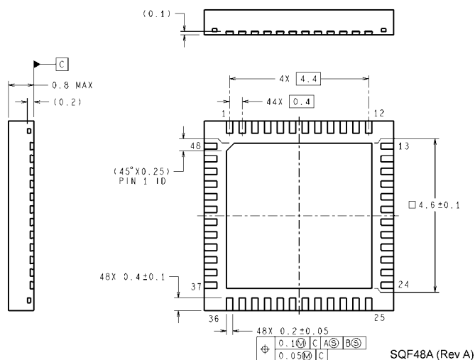
SQF48A Package: 6x6x0.8mm 48-Pin LLP Package with 0.4mm Pitch
