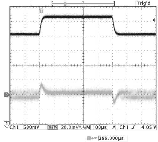
Line Transient Response Vin = 3 – 3.6 V, Vout = 3.3 V, 250 mA load
