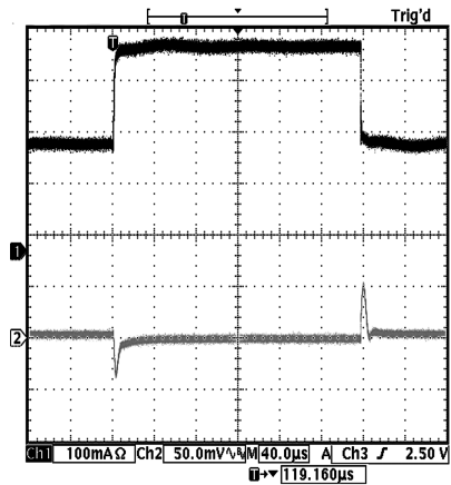
BUCK 1 Load Transient Response V_{IN} = 4.2V , V_{OUT} = 1.2V , I_{LOAD} = 200-400mA (PWM Mode)
