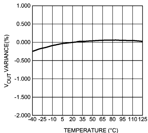
Output Voltage Change vs Temperature (LDO2) V_{in} = 4.3\text{V} , V_{out} = 1.8\text{V} , 100 mA load
