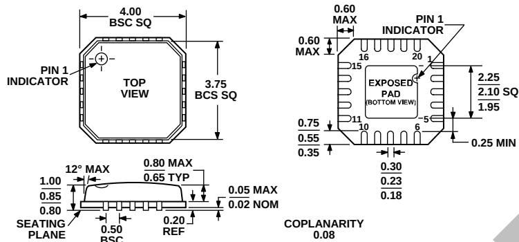
Figure 19. 20-Lead Lead Frame Chip Scale Package [LFCSP_VQ] 4 mm x 4 mm Body, Very Thin Quad (CP-20-1) Dimensions shown in millimeters
