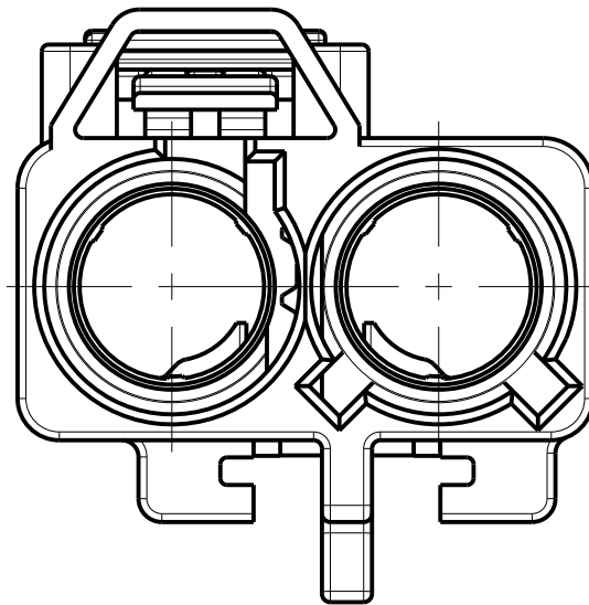
DETAIL K SCALE 4:1
