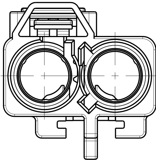
DETAIL H SCALE 4:1
