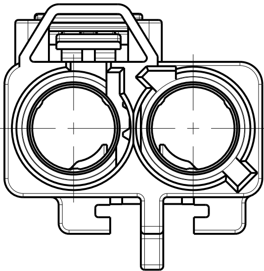
DETAIL G SCALE 4:1
