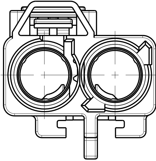
DETAIL N SCALE 4:1
