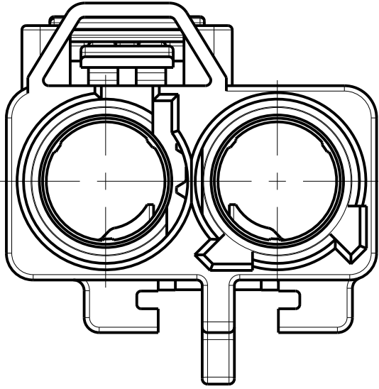
DETAIL M SCALE 4:1
