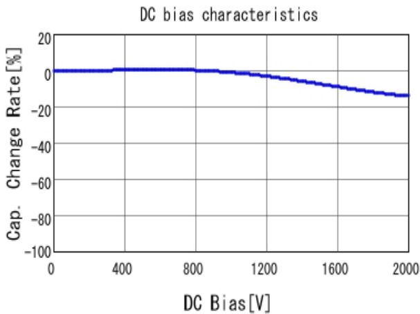
■ GR442QR73D181KW01 C-DC bias capchange, 25.0degC, AC1V
