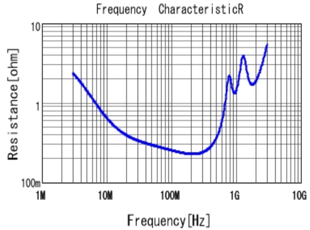
■ GR442QR73D181KW01 R DC0V, 25degC
