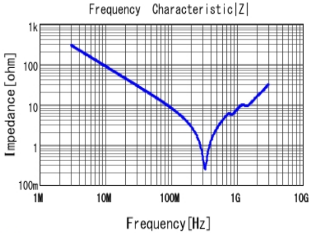
■ GR442QR73D181KW01 |Z| DC0V, 25degC
