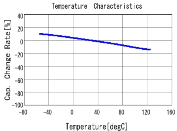
■ GR442QR73D181KW01 C-Temp. capchange, DC0V, AC1Vrms
