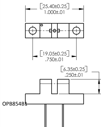
OPB854A3/OPB854B3 - Housing
