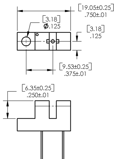
OPB854A2/OPB854B2 - Housing
