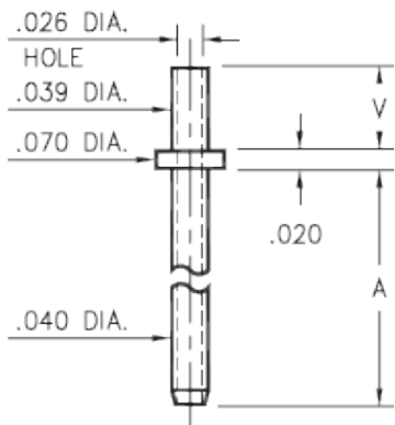
322X-X-00-XX-00-00-08-0 Swage mount in .043 hole
