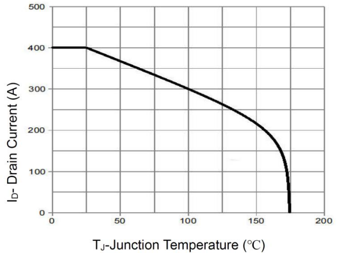
Current De-rating
