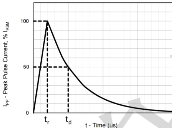
Fig.3 - Pulse Waveform
