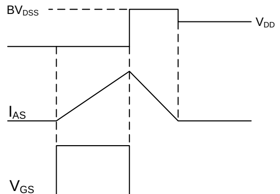
Fig.12 EAS Waveform
