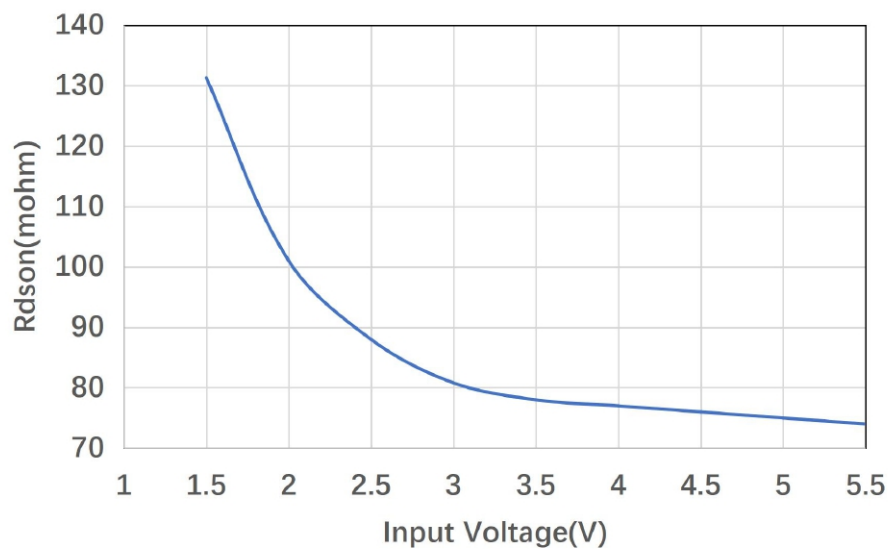
R_{ON} vs. V_{IN} ( V_{EN}=V_{IN} , I_{LOAD}=200\text{mA} )
