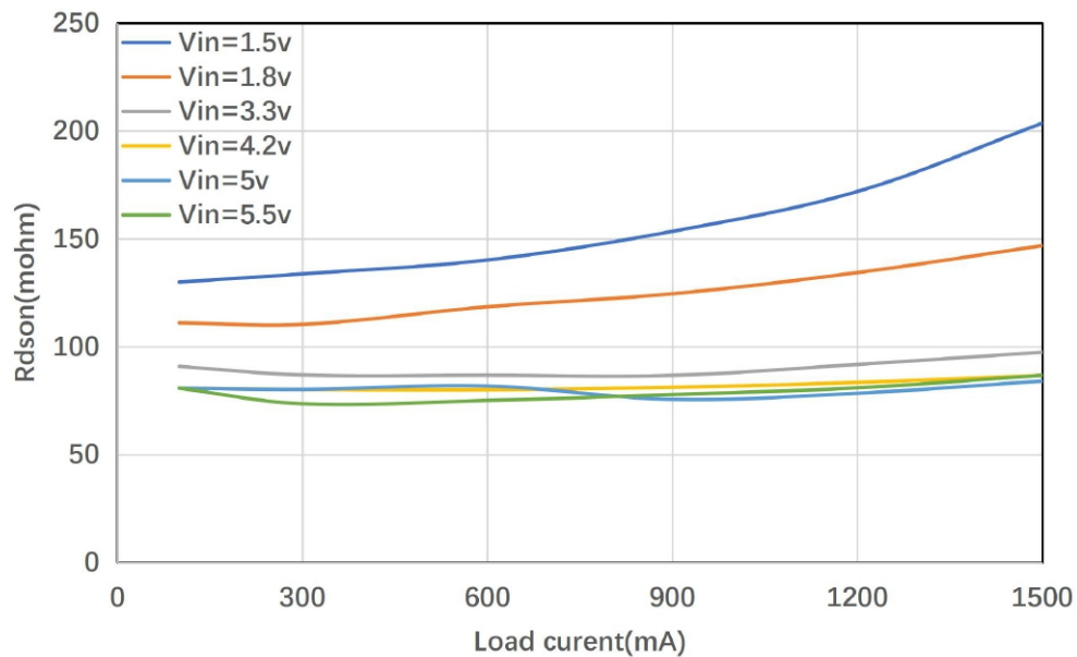
R_{ON} vs. Load current ( V_{EN}=H )
