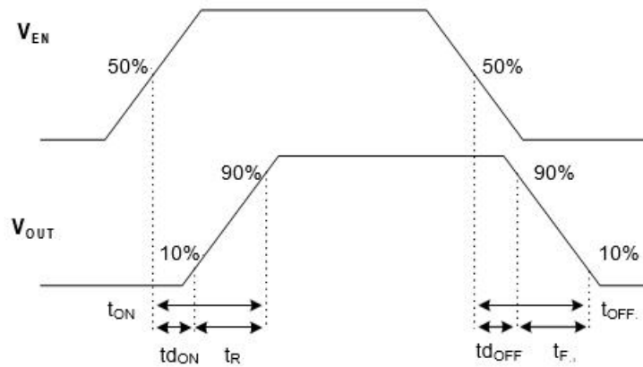
Timing Diagram
