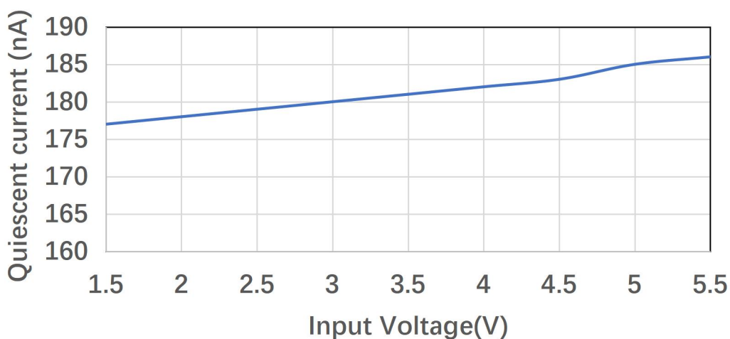
Quiescent current vs. V_{IN} ( V_{EN}=H, NO\ LOAD )
