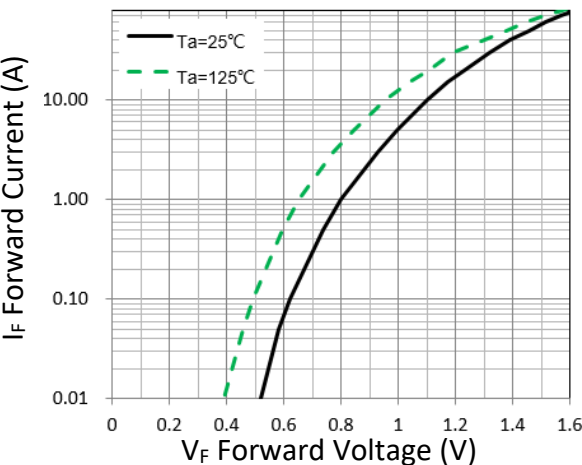
Figure 1. Forward Characteristic(typ.)
