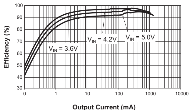
Efficiency vs. Output Current ( V_{OUT} = 3.3V )
