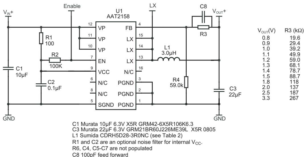
Figure 1: AAT2158 Evaluation Schematic.
