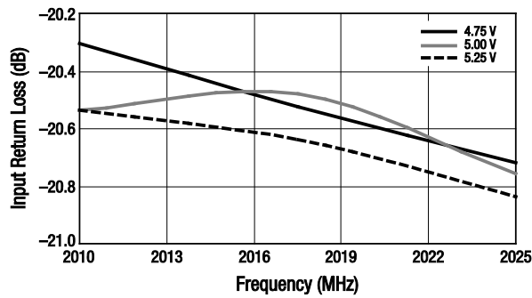
Figure 56. Input Return Loss vs Frequency Over Voltage
