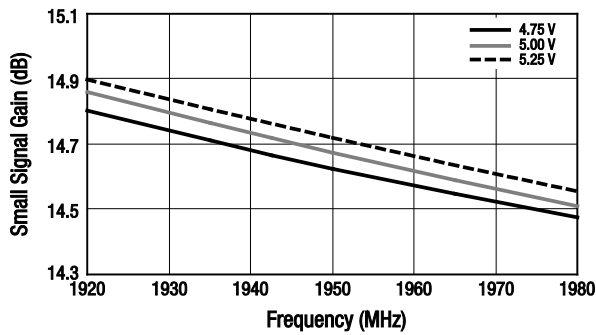
Figure 47. Small Signal Gain vs Frequency Over Voltage
