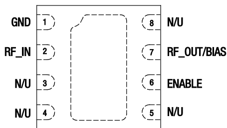
Figure 2. SKY65095-360LF Pinout – 8-Pin DFN Package (Top View)
