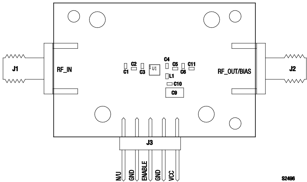
Figure 67. Evaluation Board Assembly Drawing
