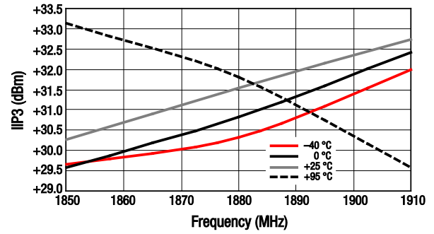
Figure 38. IIP3 vs Frequency Over Temperature
