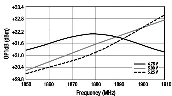
Figure 36. OP1dB vs Frequency Over Voltage
