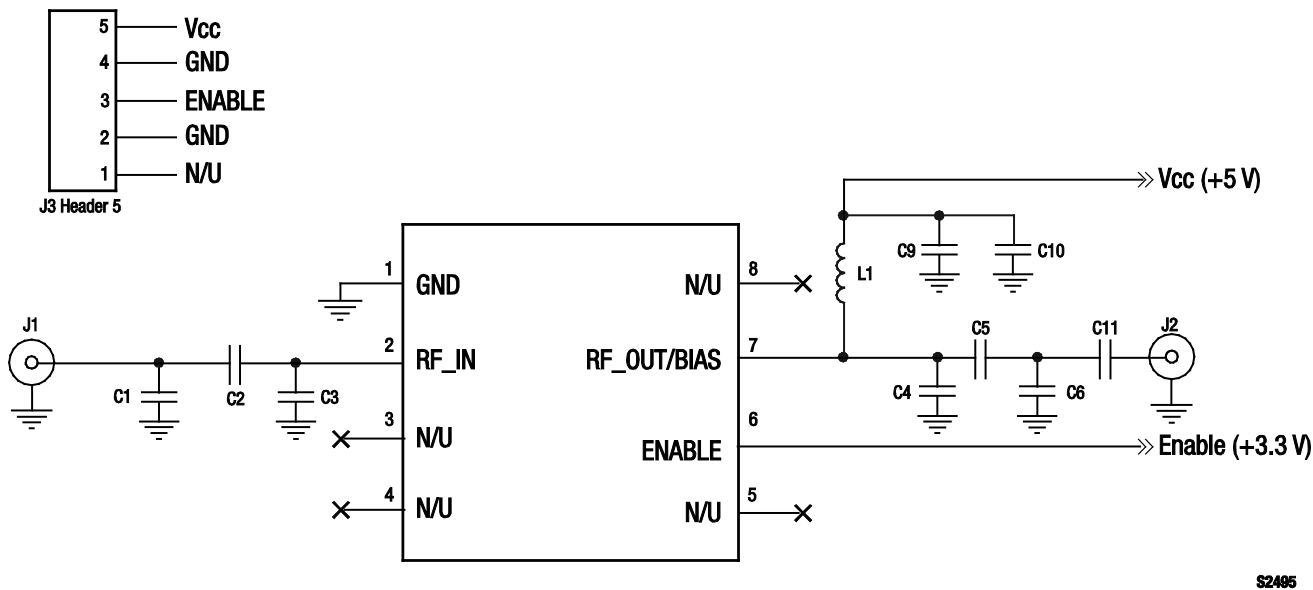
Figure 70. SKY65095-360LF Evaluation Board Schematic
