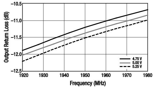
Figure 46. Output Return Loss vs Frequency Over Voltage
