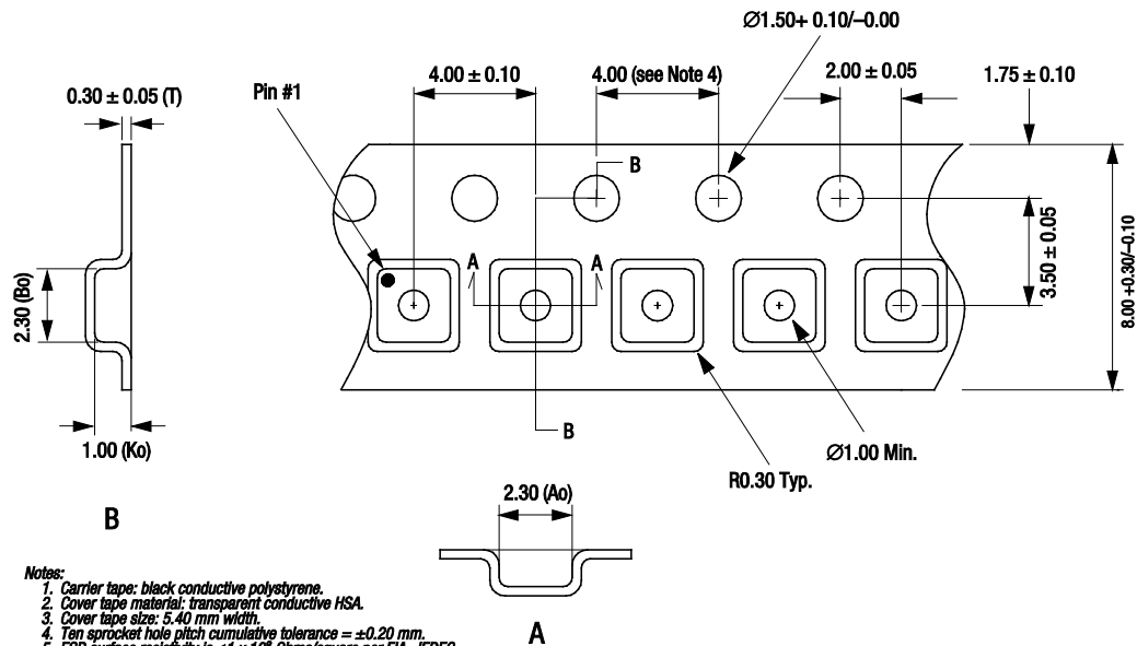
Figure 73. SKY65095-360LF Tape and Reel Dimensions
