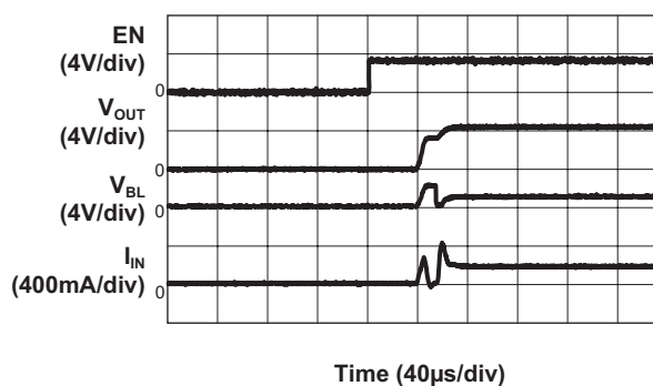
Turn-On to 1.5x Mode Backlight ( V_{IN} = 3.3V ; 30mA/ch)
